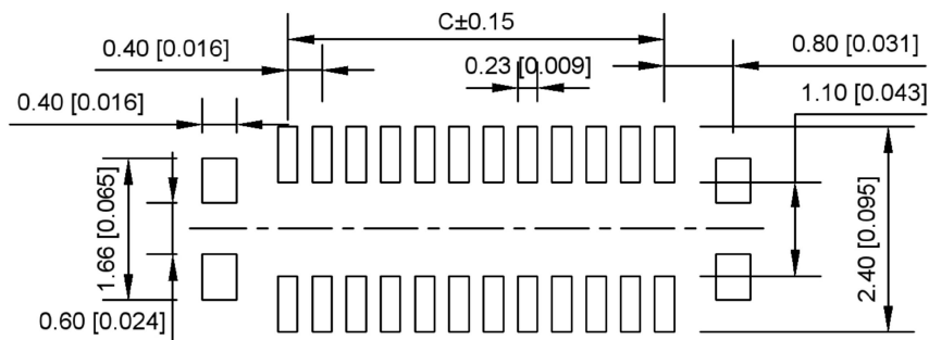
RECOMMENDED PCB LAYOUT CONNECTOR SIDE
