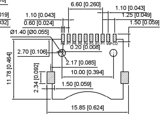
Recommended P.C.B Layout(Top Side)
