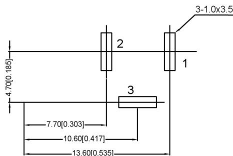
PCB LAYOUT TOP VIEW TOLERANCES:±0.05
