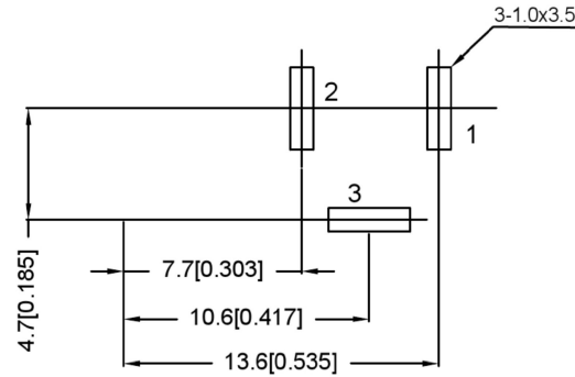
PCB LAYOUT TOP VIEW TOLERANCES:±0.05
