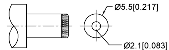
MATING PLUG Jack Insertion Depth: 9.0 mm
