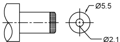
MATING PLUG Jack Insertion Depth: 9.0 mm
