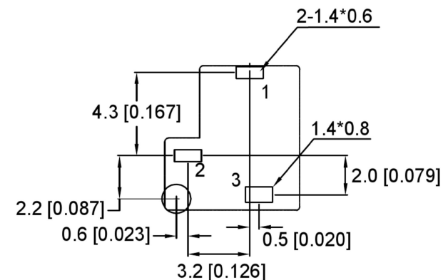
PCB LAYOUT TOP VIEW TOLERANCES: ±0.05
