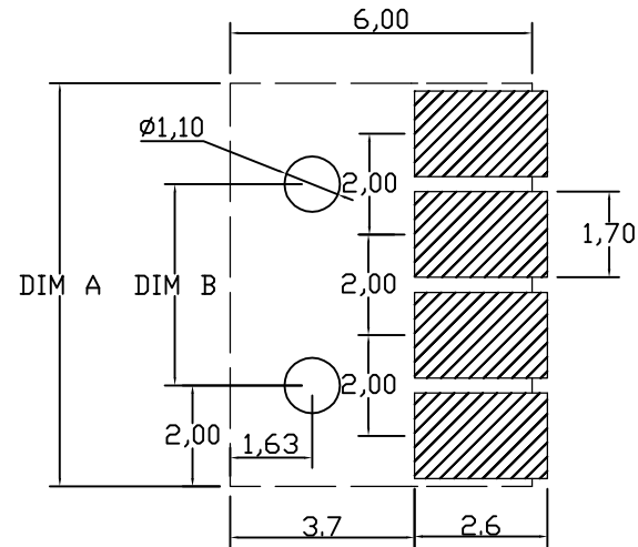
RECOMMENDED PCB LAYOUT TOP VIEW (. XX \pm 0.05)
