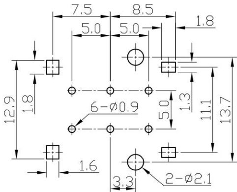
P. C. B HOLE LAYOUT
