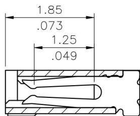
SEC.: J-J
