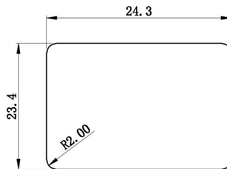
PANEL CUT-OUT
