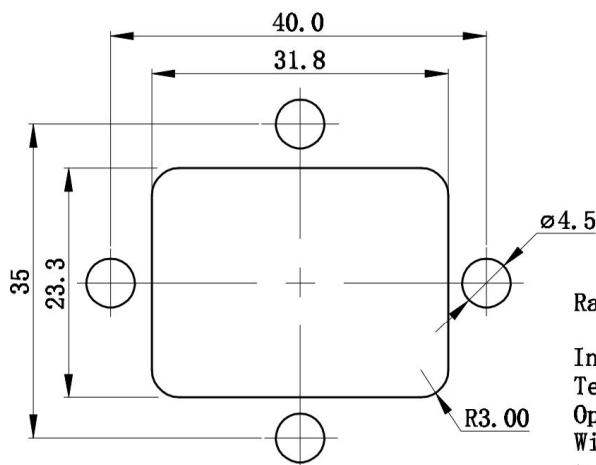
PANEL CUT-OUT
