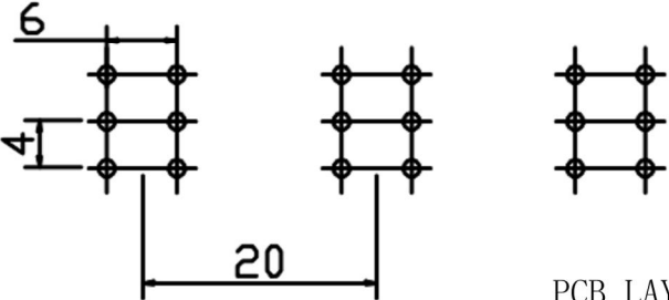
PCB LAYOUT
