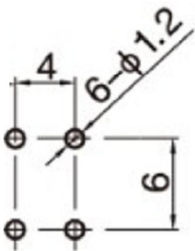
PCB LAYOUT
