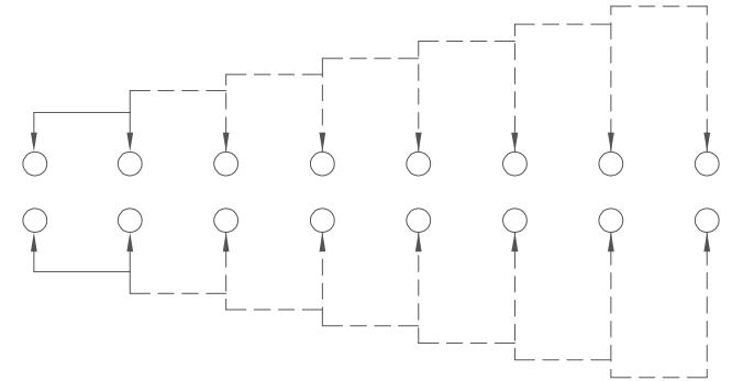
SCHEMATIC (NON-SHORTING)
