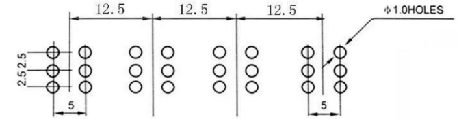
PCB LAYOUT
