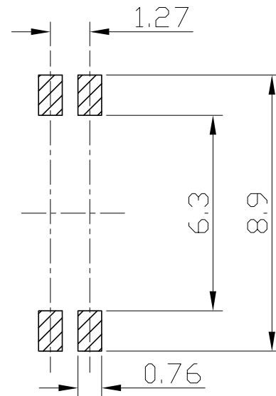
P. C. B LAYOUT
