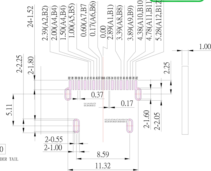
P.C.B LAYOUT MOUNTING PATTERN
