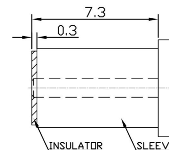
MATE PLUG
