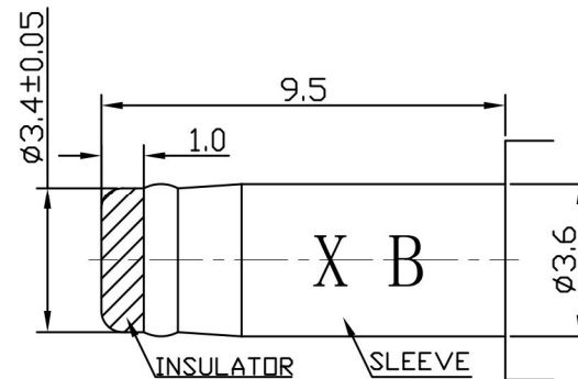
MATE PLUG
