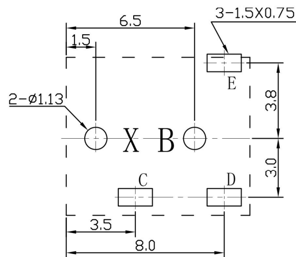
P、B、C LAYOUT
