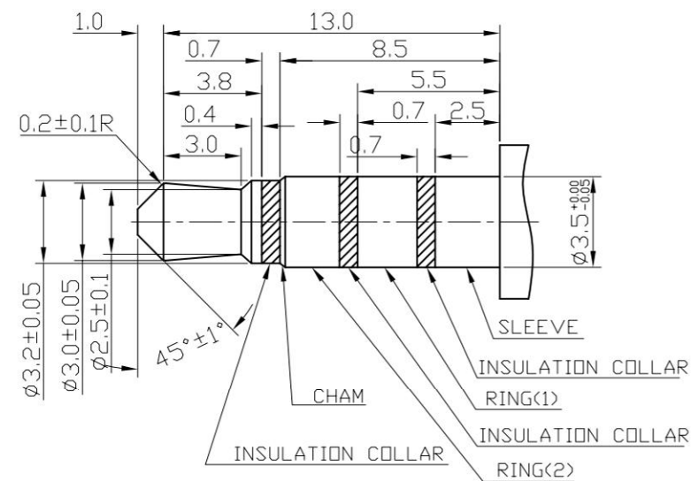
MATE PLUG
