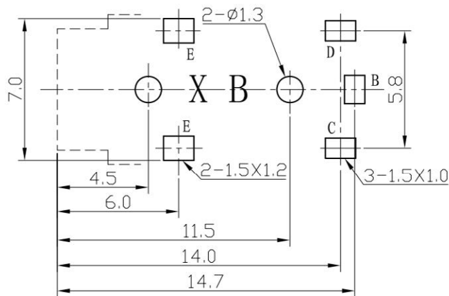
HOLE LAYOUT (BOTTOM VIEW)
