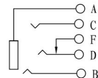
ST-053B SCHEMATIC
