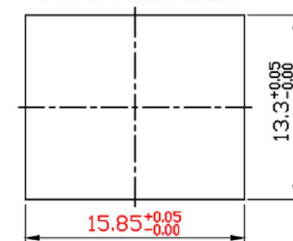
Mounting Hole Dimensions
