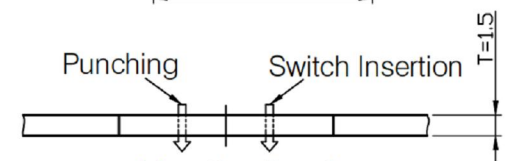
Mounting Panel Hole Dimensions
