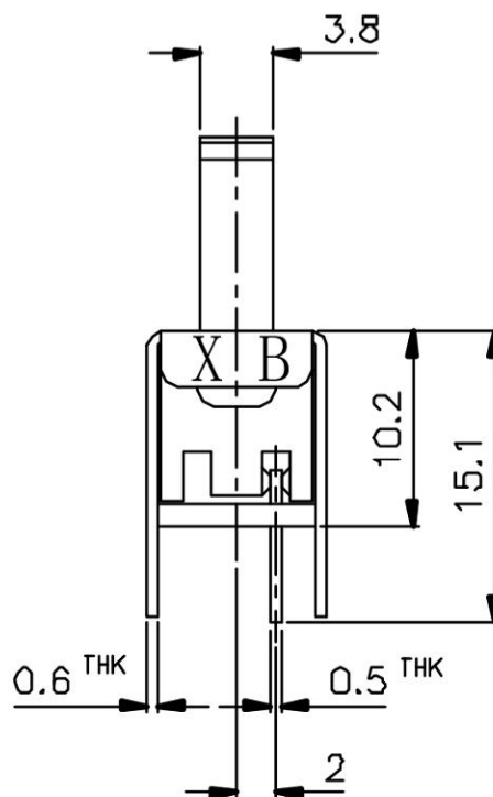
SLIDE SWITCH 1P4T
