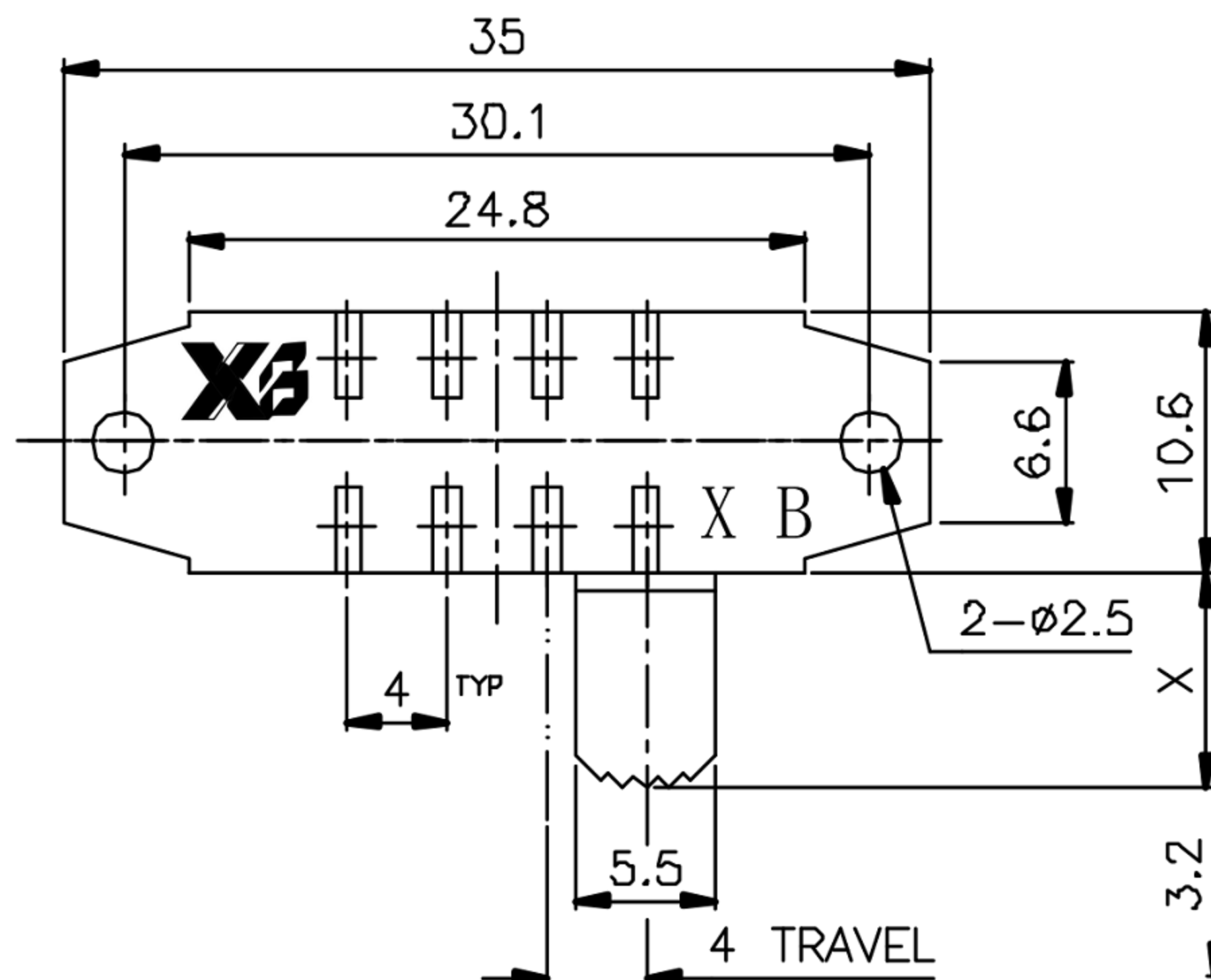
SIDE KNOB SLIDE SWITCH 2P4T
