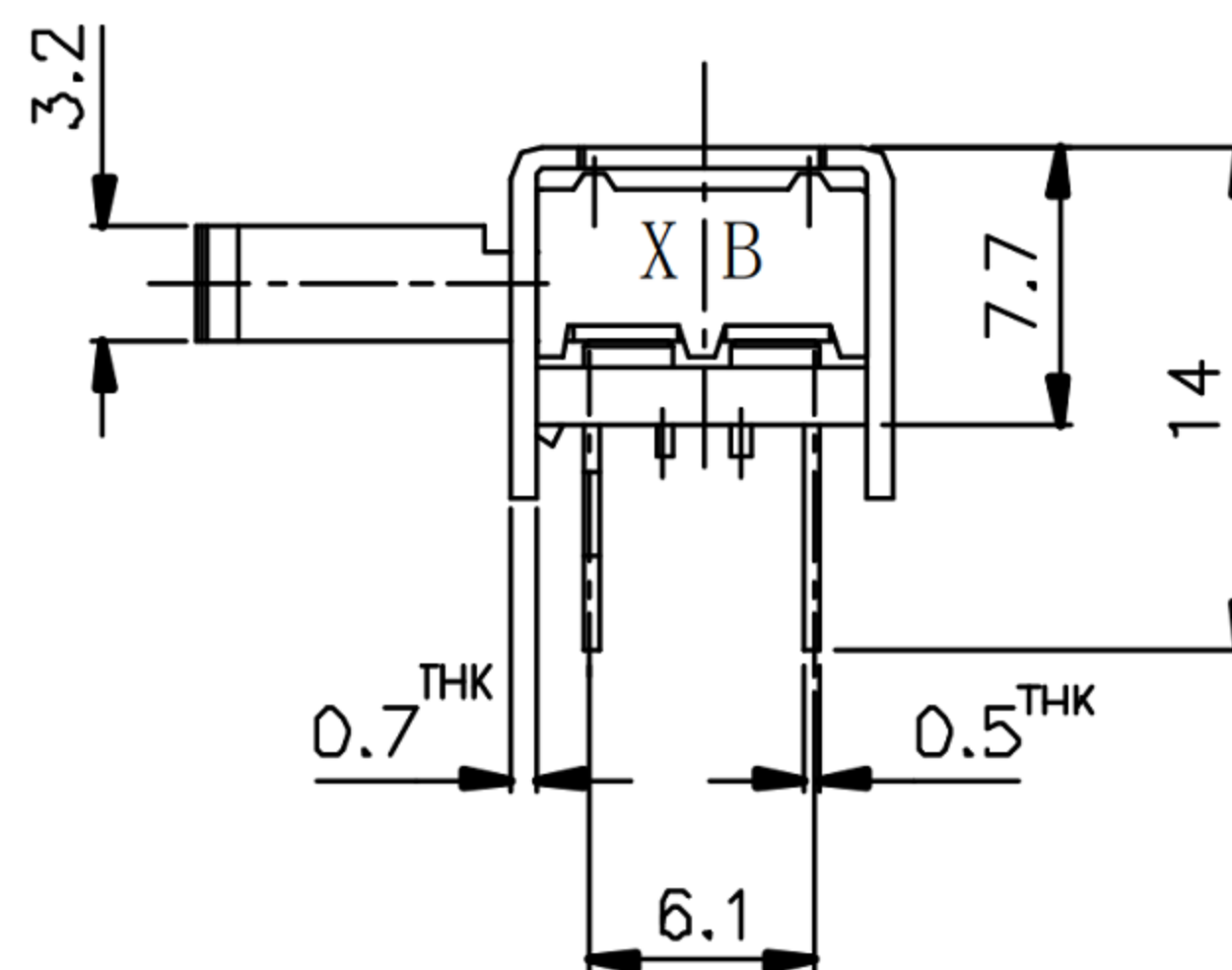
SIDE KNOB SLIDE SWITCH 2P4T
