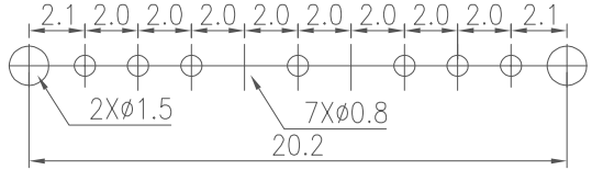
P.C.B LAYOUT TOP VIEW
