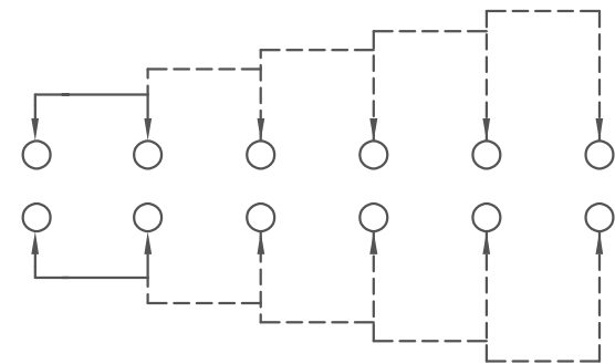
SCHEMATIC (NON-SHORTING)
