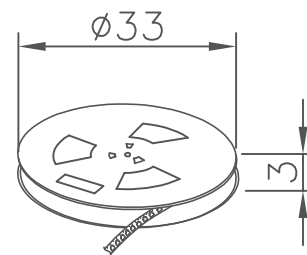
载带(400pcs/盘)
