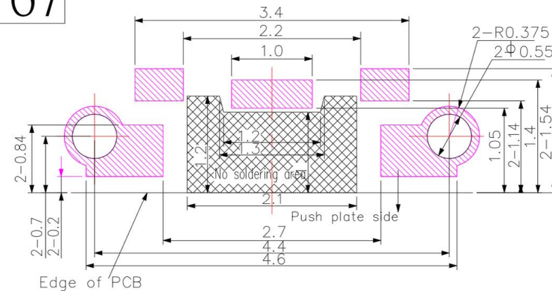
PCB LAYOUT
