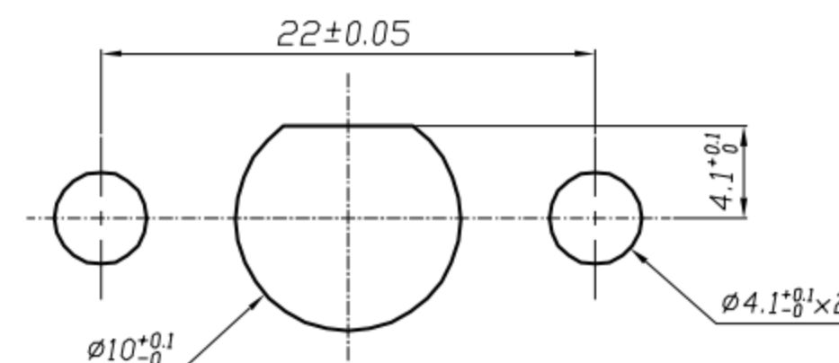
PANEL CUTOUT
