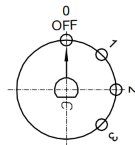
CIRCUIT DIAGRAM
