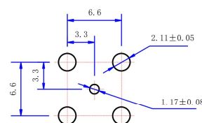
PCB HOLE CONFIGURATION RECOMMENDED PANEL CUTOUTS
