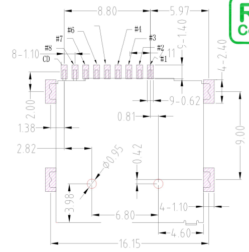
PCB LAYOYT
