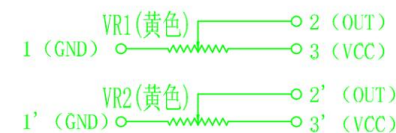
CIRCUIT:VR
