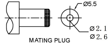
MATING PLUG
