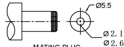
MATING PLUG
