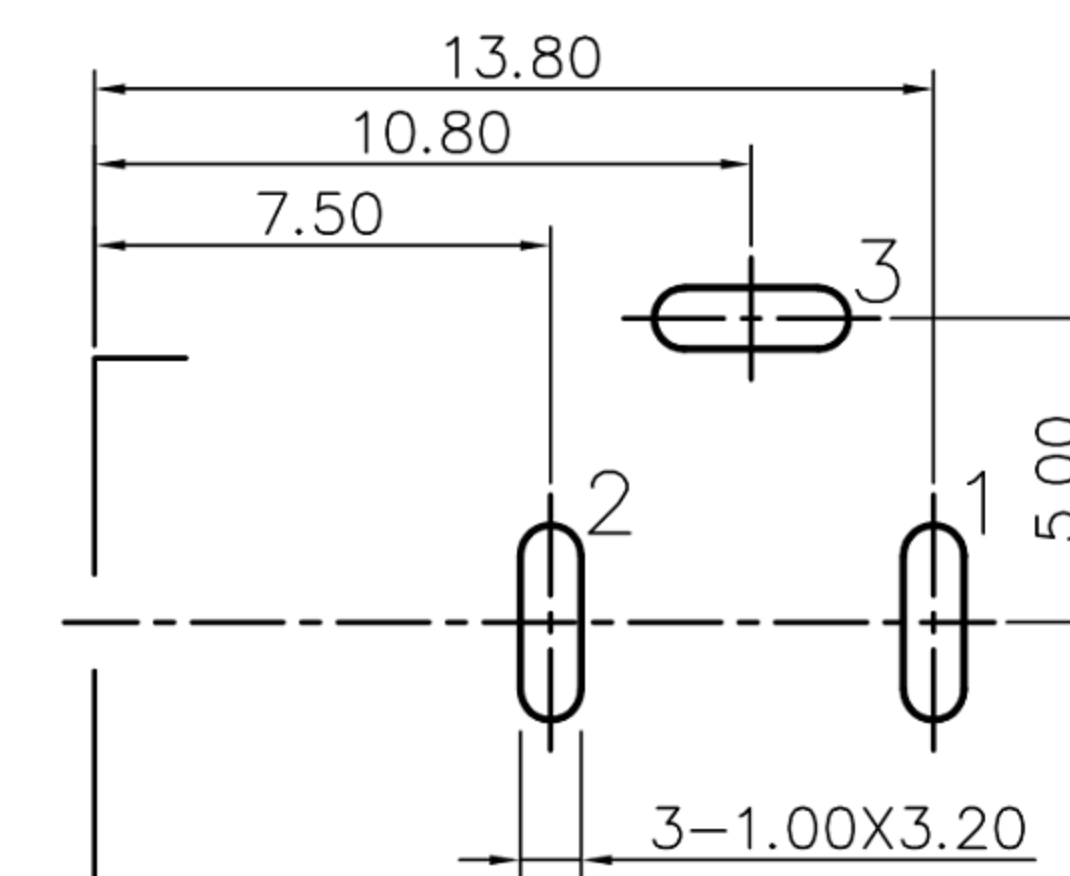
Pin Hole Layout (Jack Bottom View)
