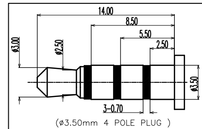
(ø3.50mm 4 POLE PLUG )
