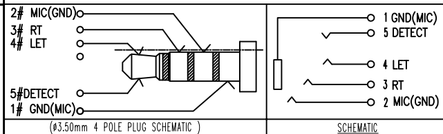
(ø3.50mm 4 POLE PLUG SCHEMATIC )
