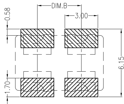
Board Layout
