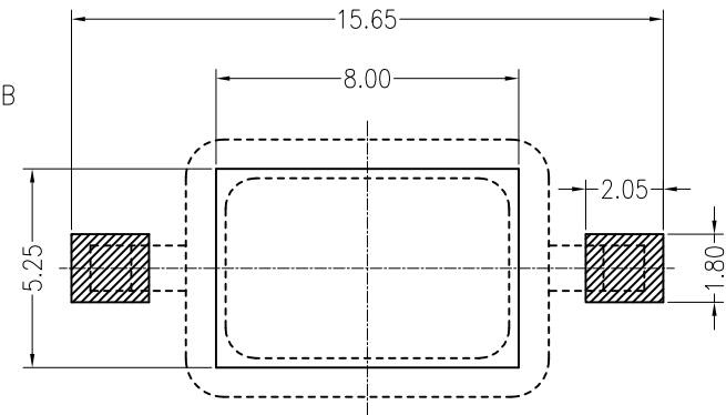
Board Layout General Tolerance:±0.05
