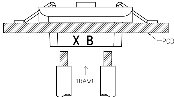
Assembly Layout
