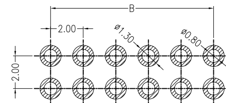
RECOMMENDED PCB LAYOUT(TOP VIEW) TOLERANCE:±0.05mm
