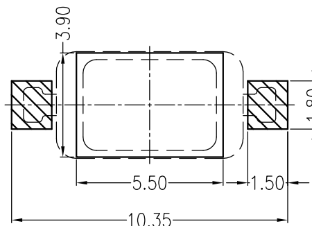
Board Layout General Tolerance: \pm 0.05
