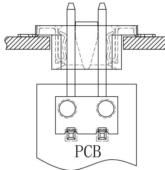
Assembly Layout
