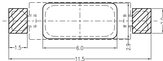
Board Layout
