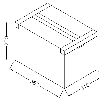
CARTON 1560 PCS
