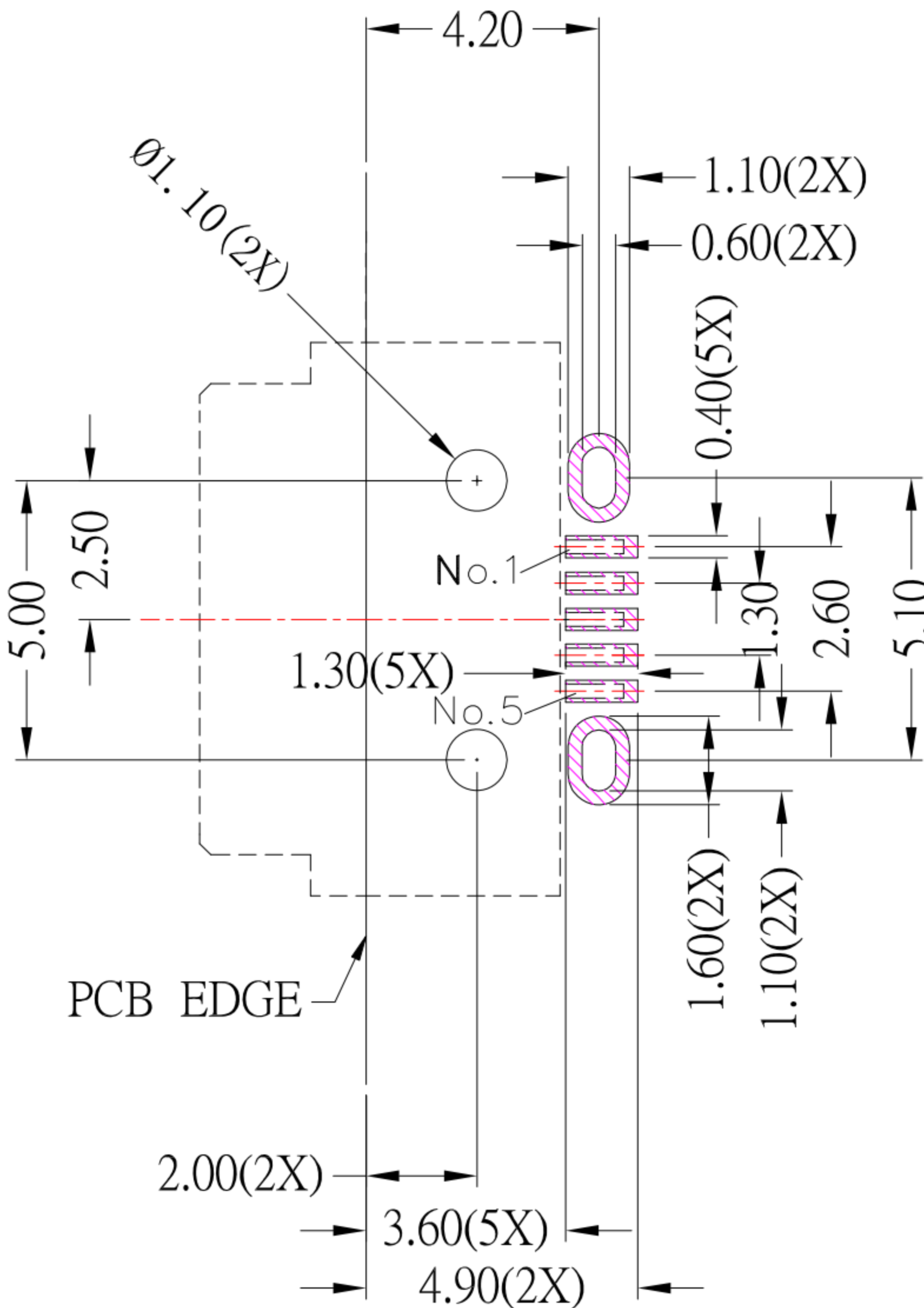
PCB LAYOUT MOUNTING PATTERN TOP VIEW
