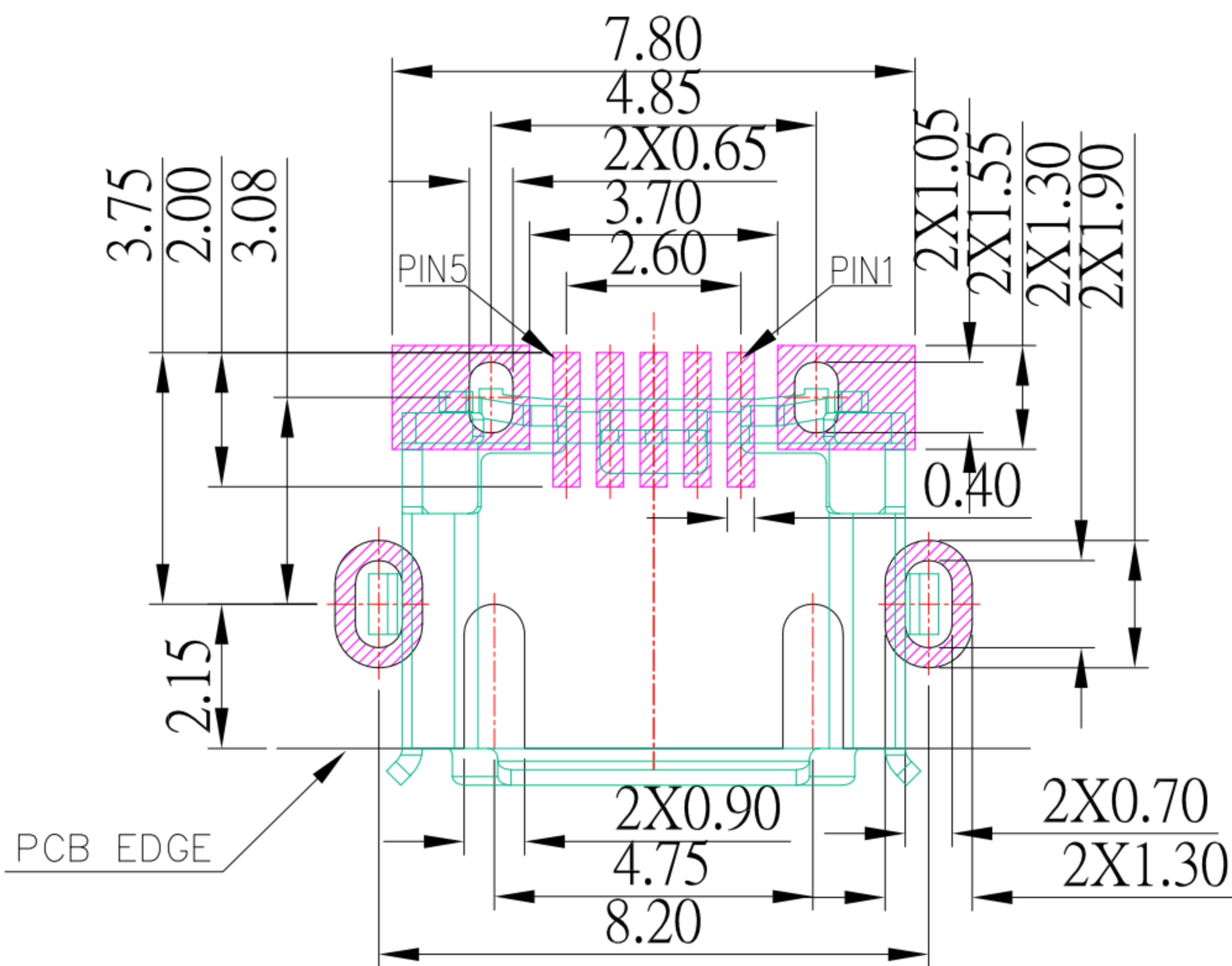
P.C.B LAYOUT MOUNTING PATTERN
