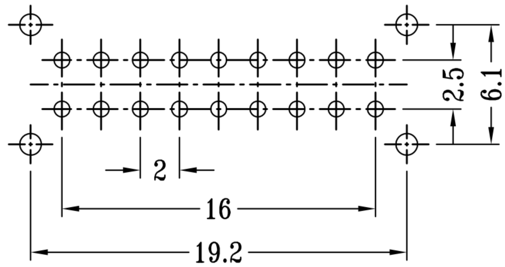
P.C.B LAYOUT BOTTOM VIEW
