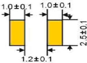
Recommended Pad Layout (mm) 建议焊盘尺寸 (毫米)
