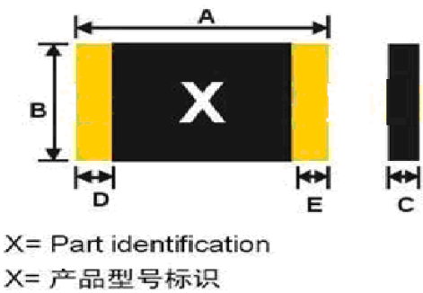
Dimension and Marking 尺寸与产品标识
