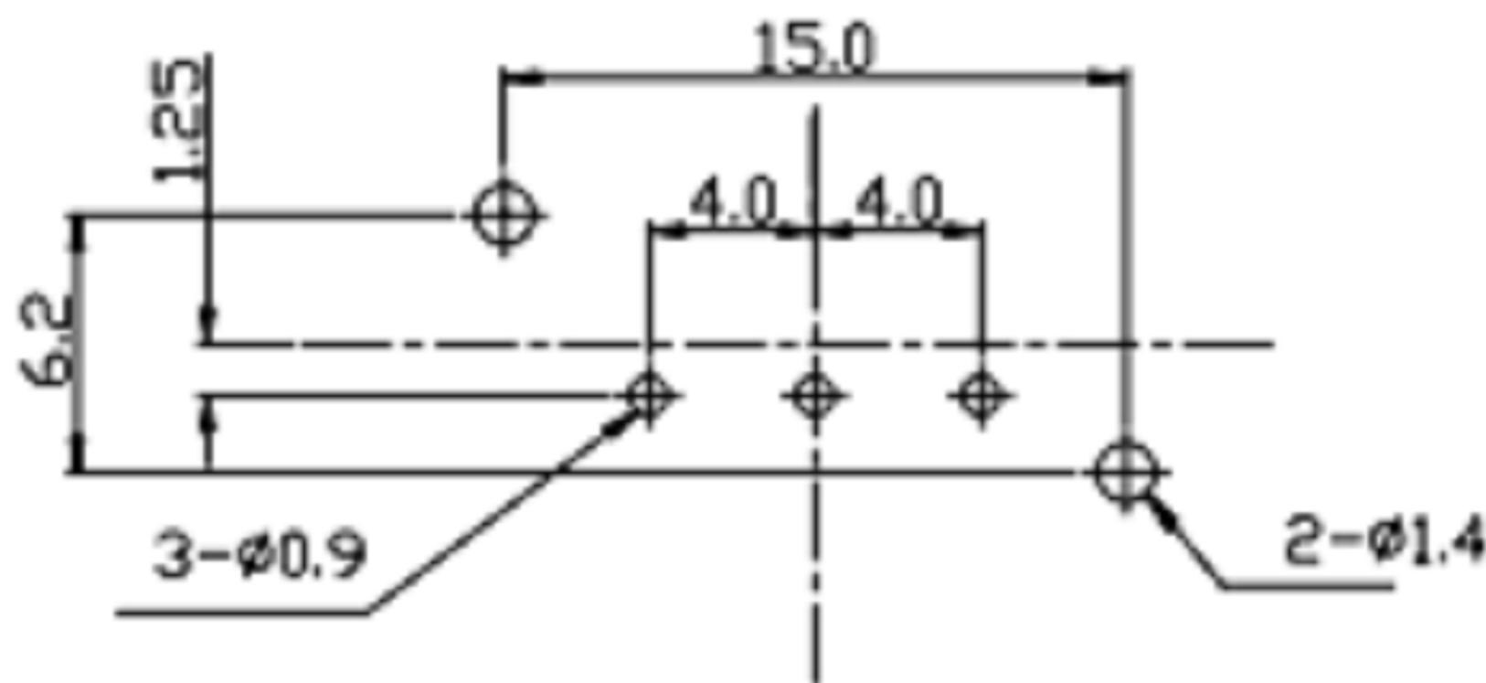
PIERCING PLAN
