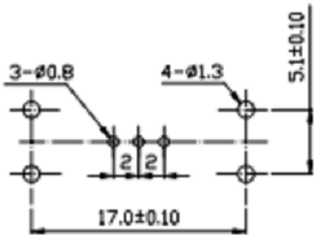
PIERCING PLAN
