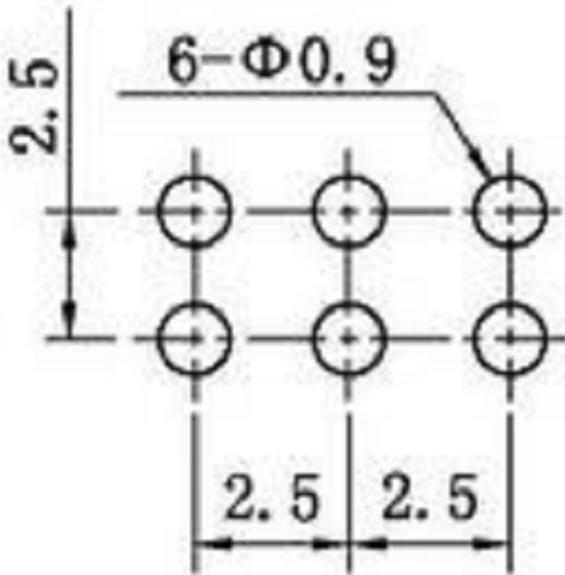
P. C. B HOLE DETAIL
